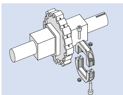
Siegling Prolink Retainer Rings provides a quick, easy and reliable solution for fixing the sprocket ( see page I-190 for details).
