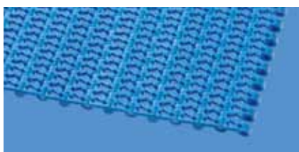
S4.1 | 21 % open | Nub Top
