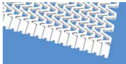
S15 | 47 % open | Grid Top
