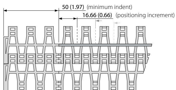
Indent configuration S2-57 GRT PMC
